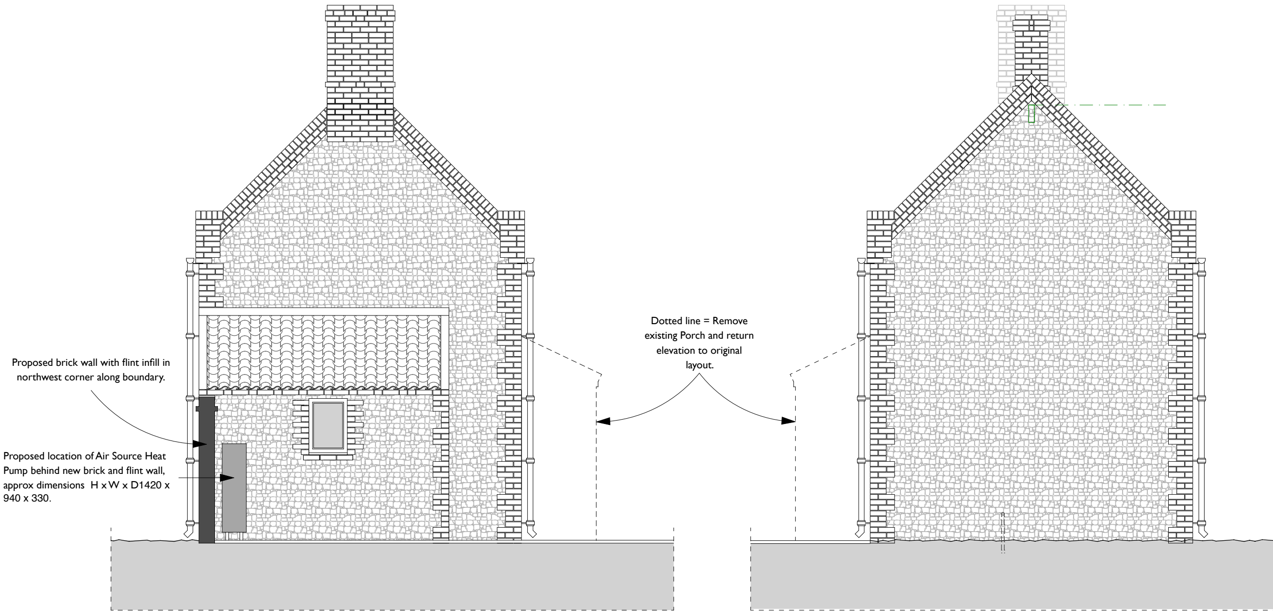
Proposed West Elevation - 1:50 @A3
