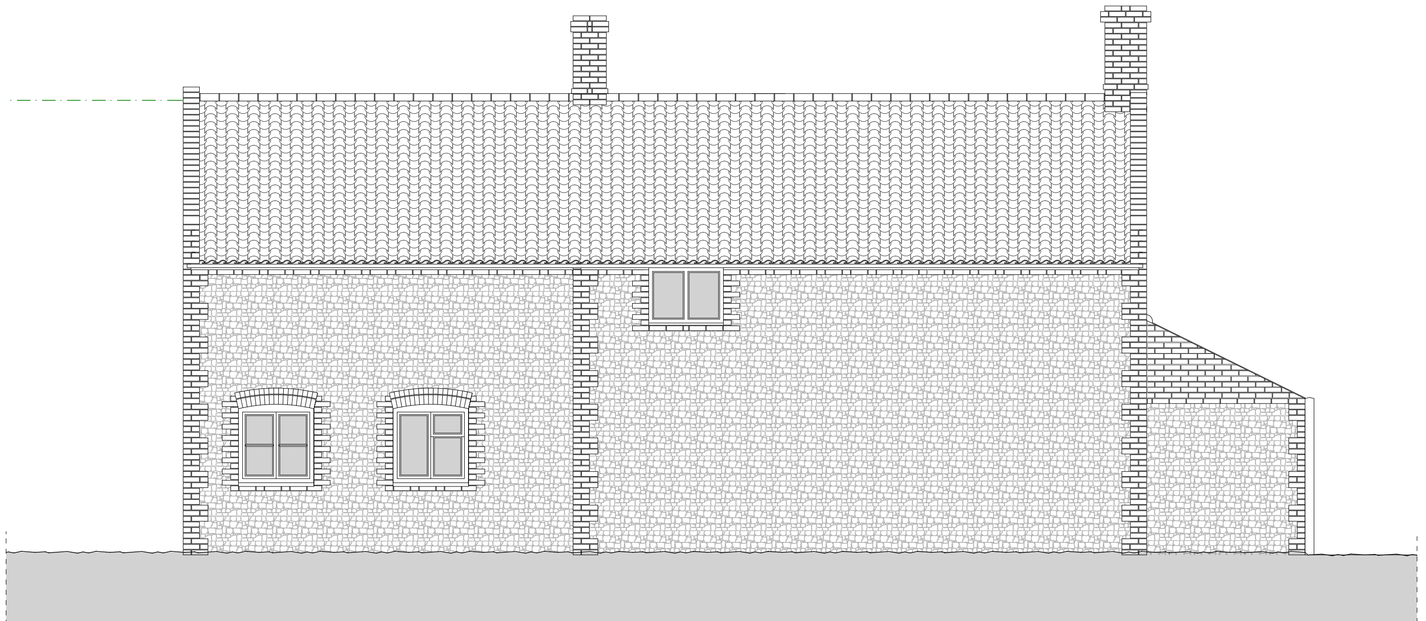
Existing North Elevation - 1:50
