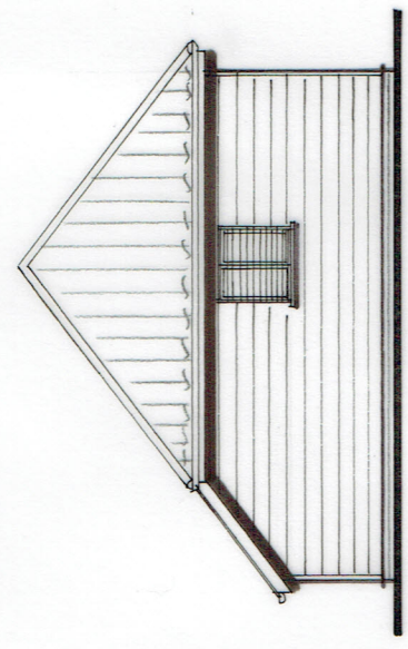
NORTH ELEVATION
