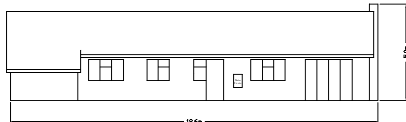
EXISTING REAR ELEVATION
