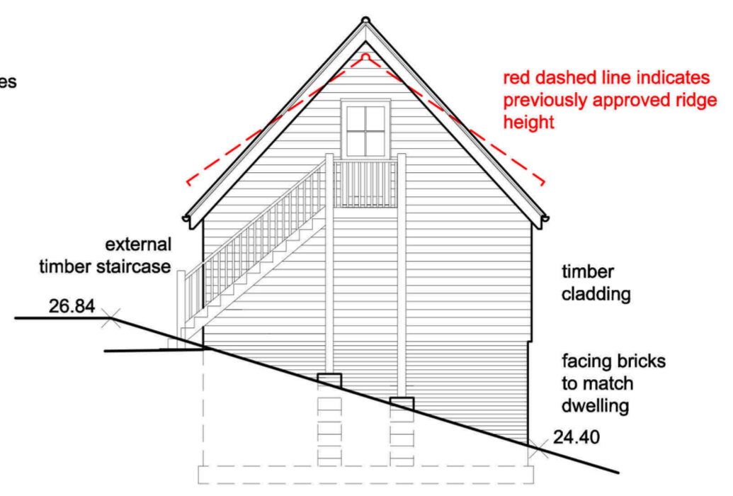
SIDE ELEVATION
