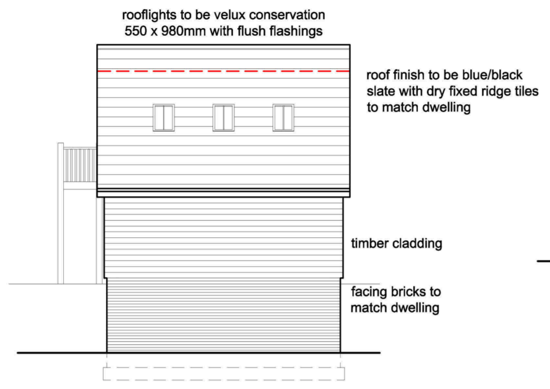
REAR ELEVATION
