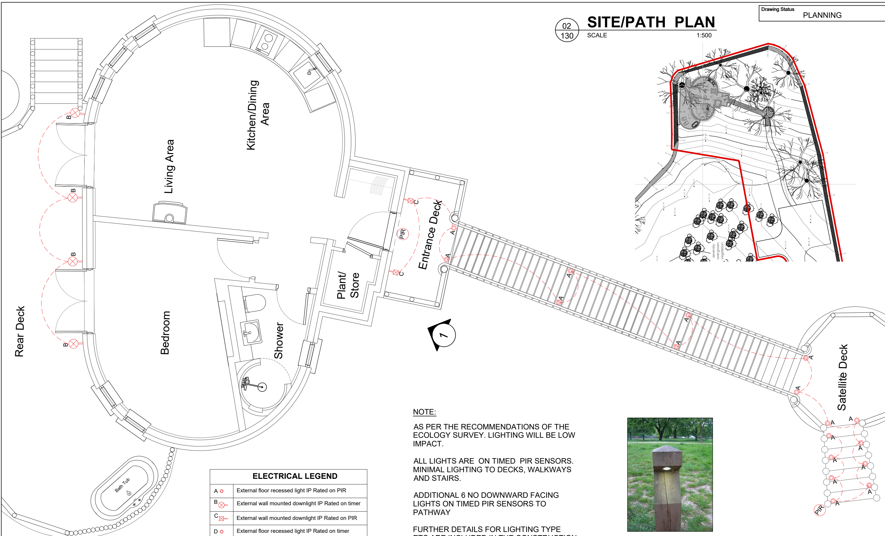
DOWNWARD FACING LIGHTS ON TIMED PIR SENSORS TO PATHWAY
