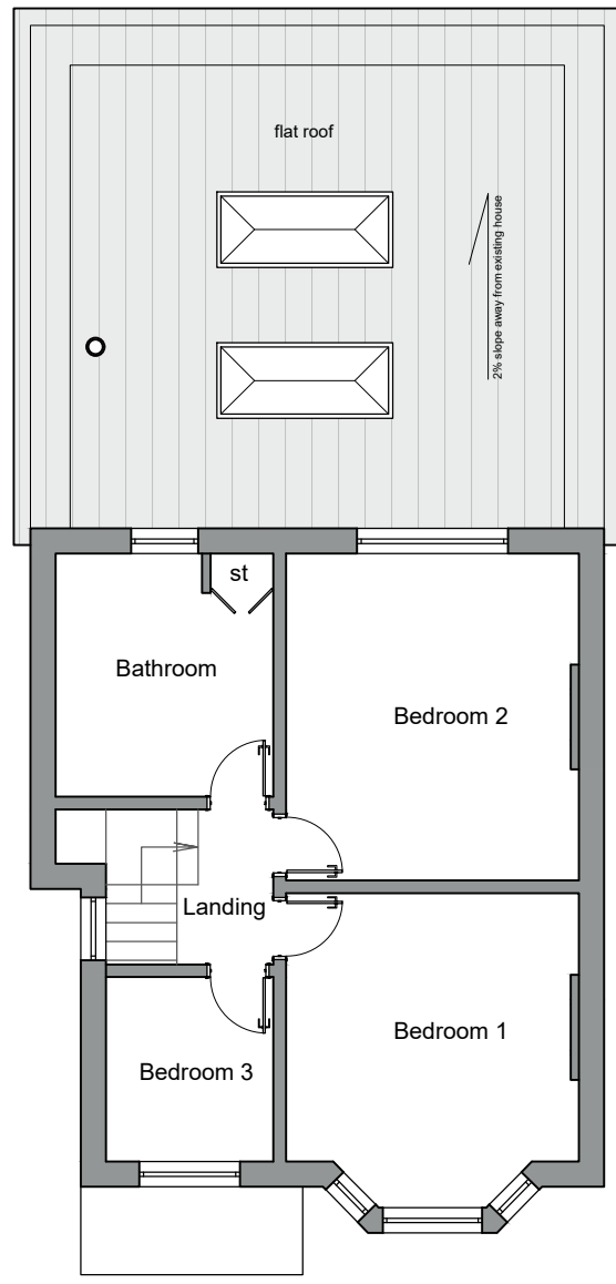
FIRST FLOOR
