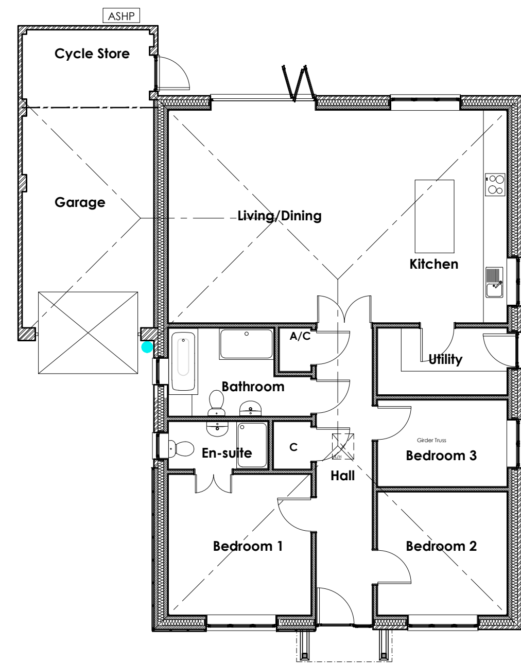
Floor Plan
