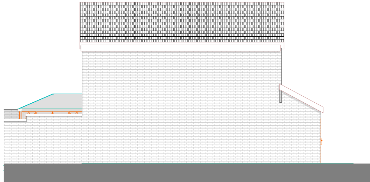
North Elevation
