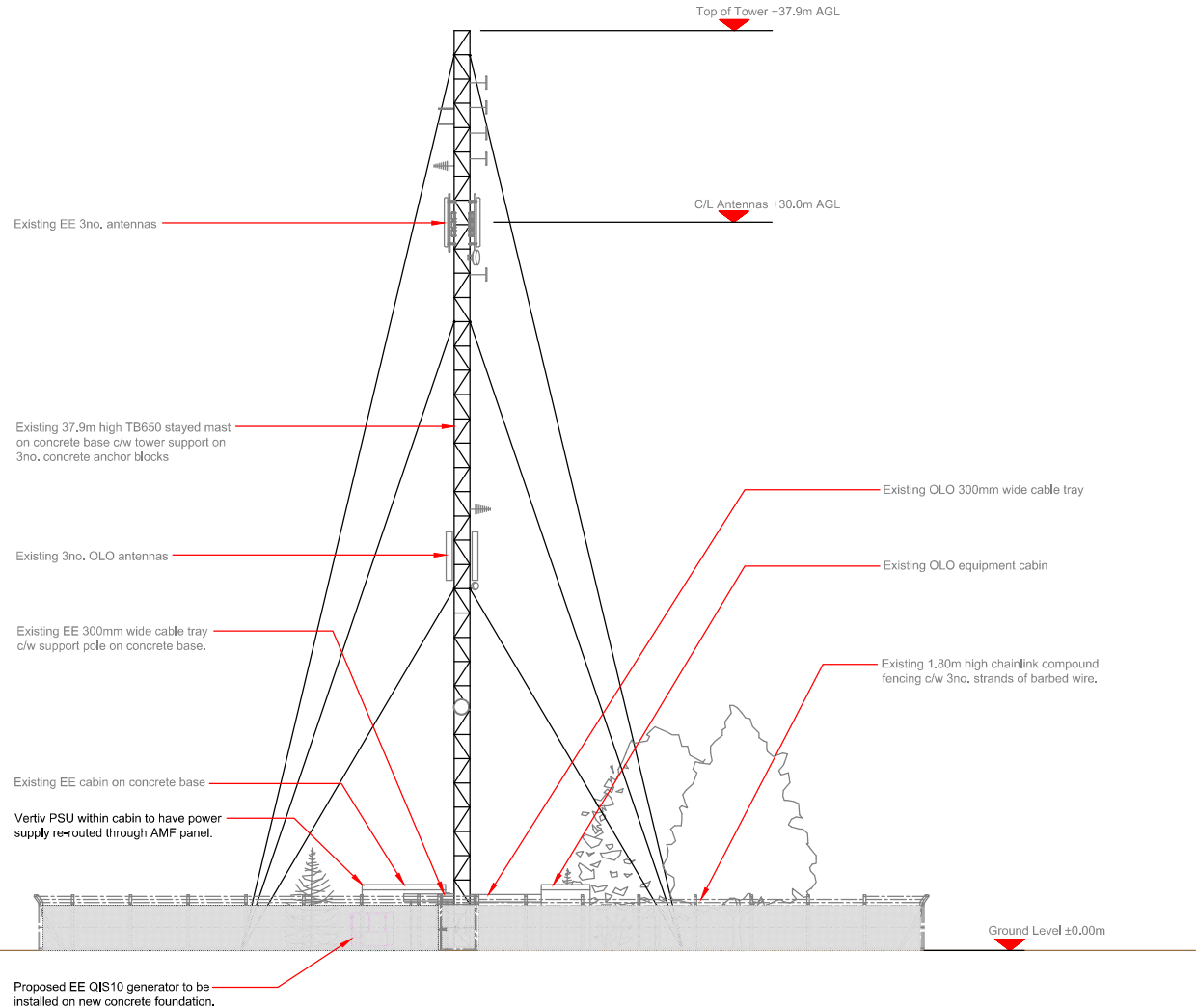
PROPOSED ELEVATION A
