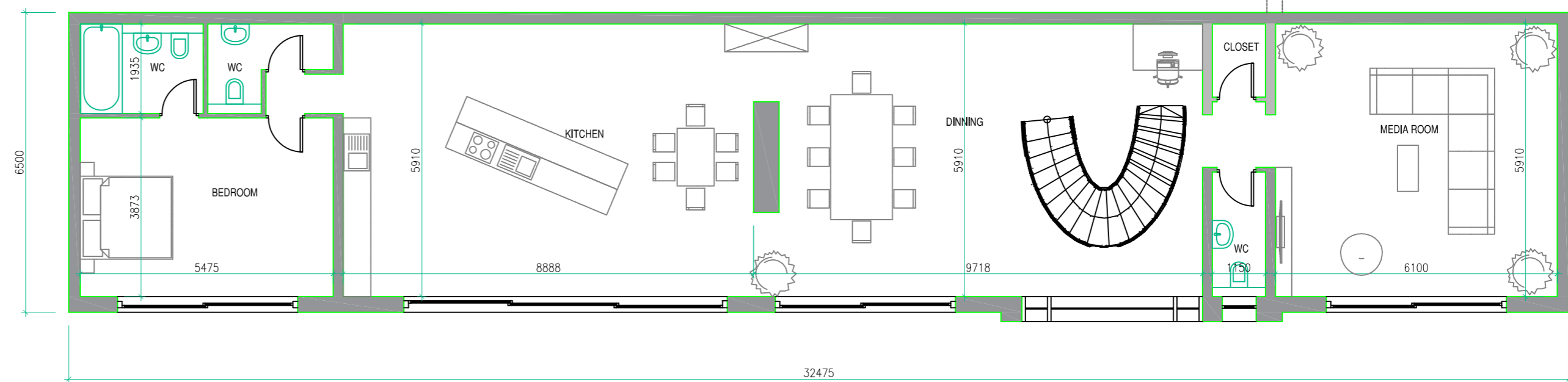
BASEMENT PLAN
