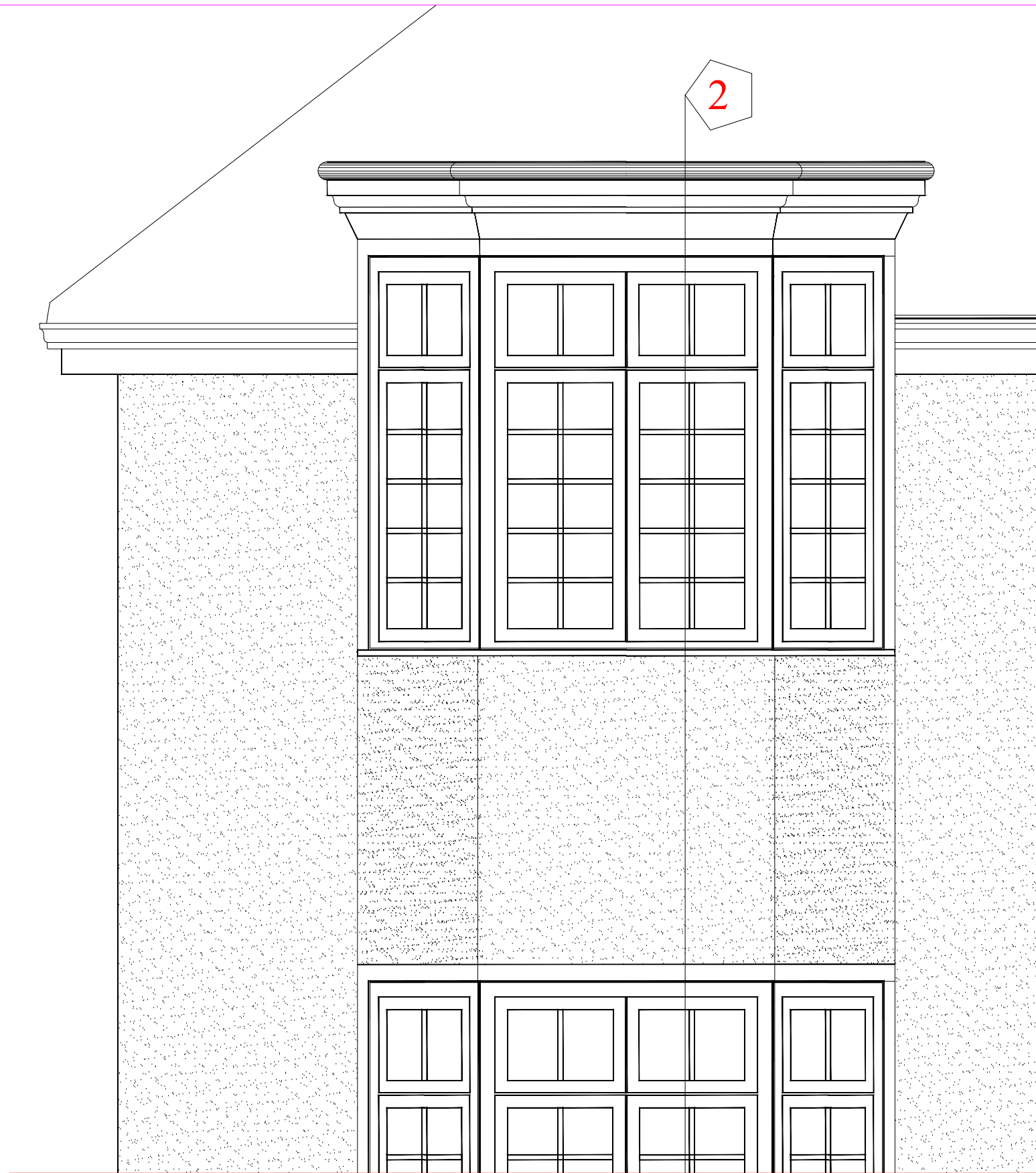
TYPICAL PROJECTED BAY WINDOW
