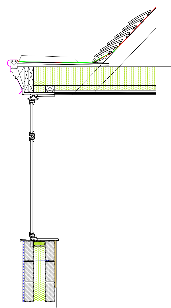
TYPICAL SECTION 2-2 OF PROJECTED BAY WINDOW
