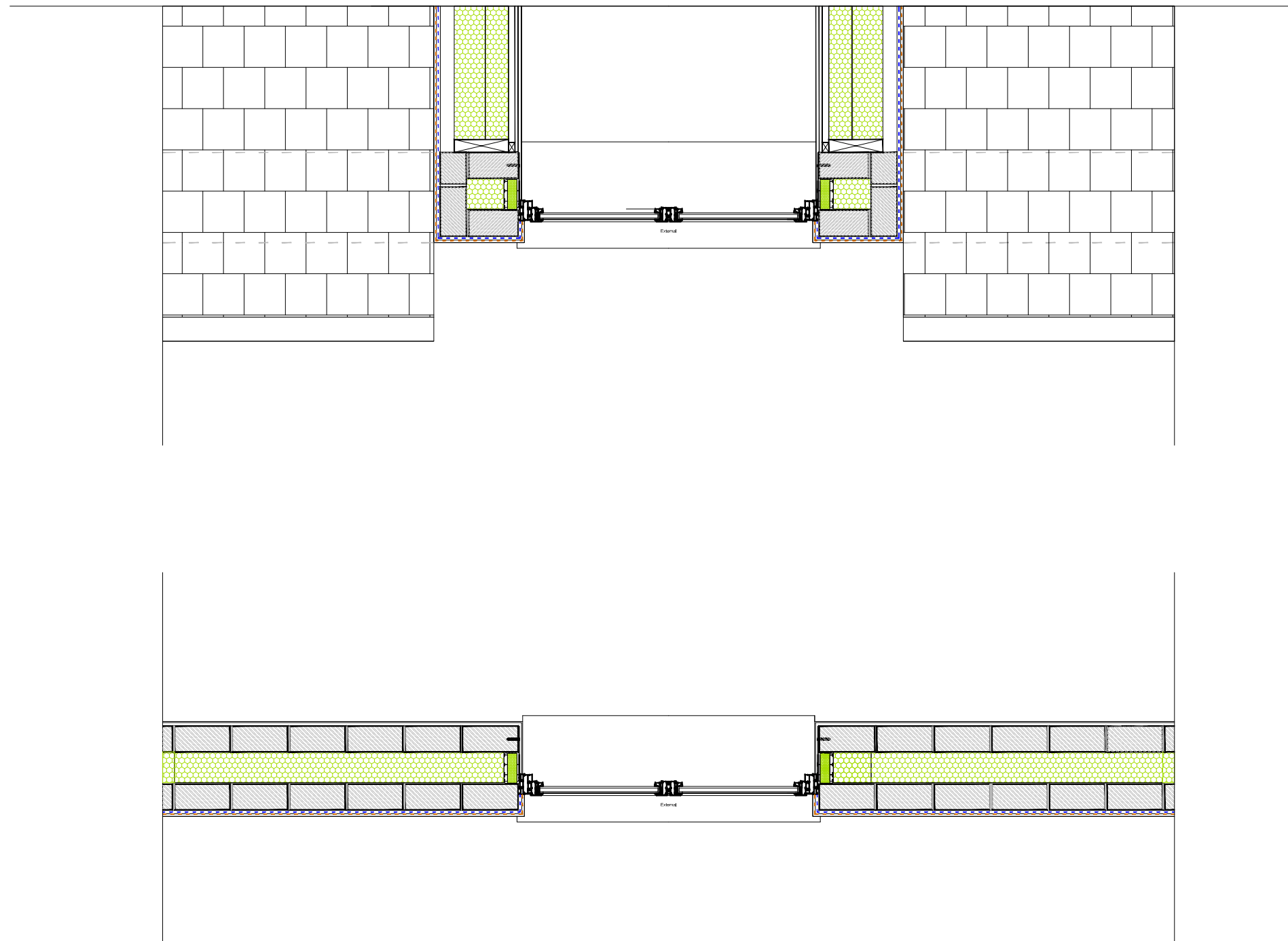
PLAN OF TYPICAL WINDOW ABOVE THE GUTTER LINE
