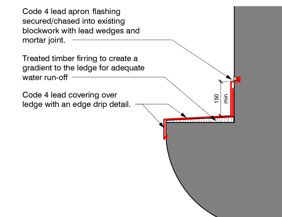
(01) Ledge flashing detail 00 Section Detail - Ledge flashing detail 1 : 10
