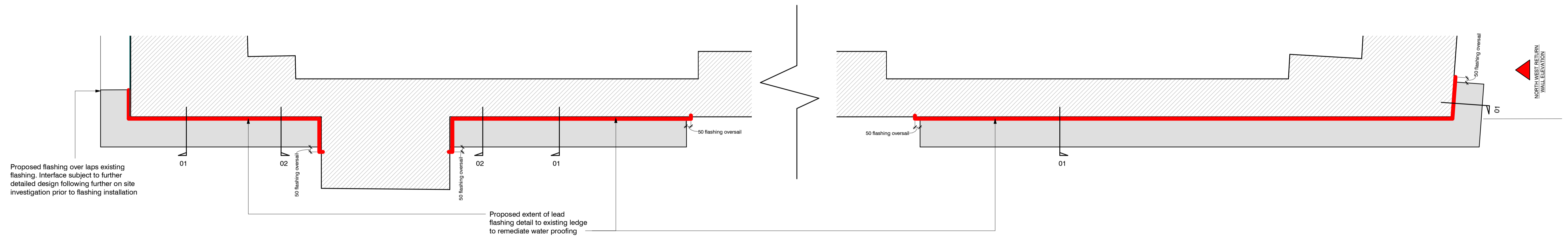
A Proposed top floor ledge - Plan 1 : 20
