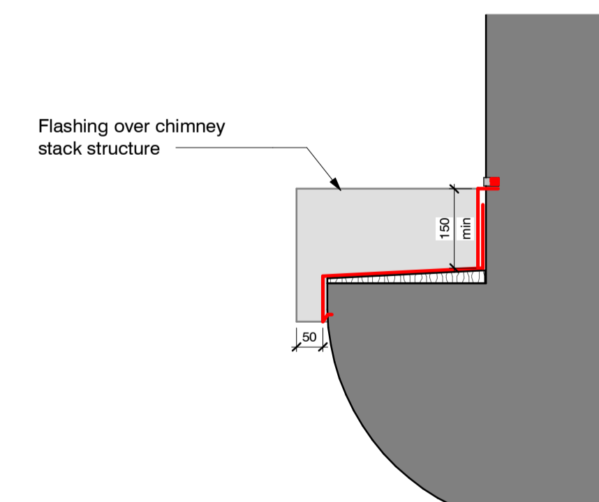
(02) Ledge flashing detail_Chimney structure
