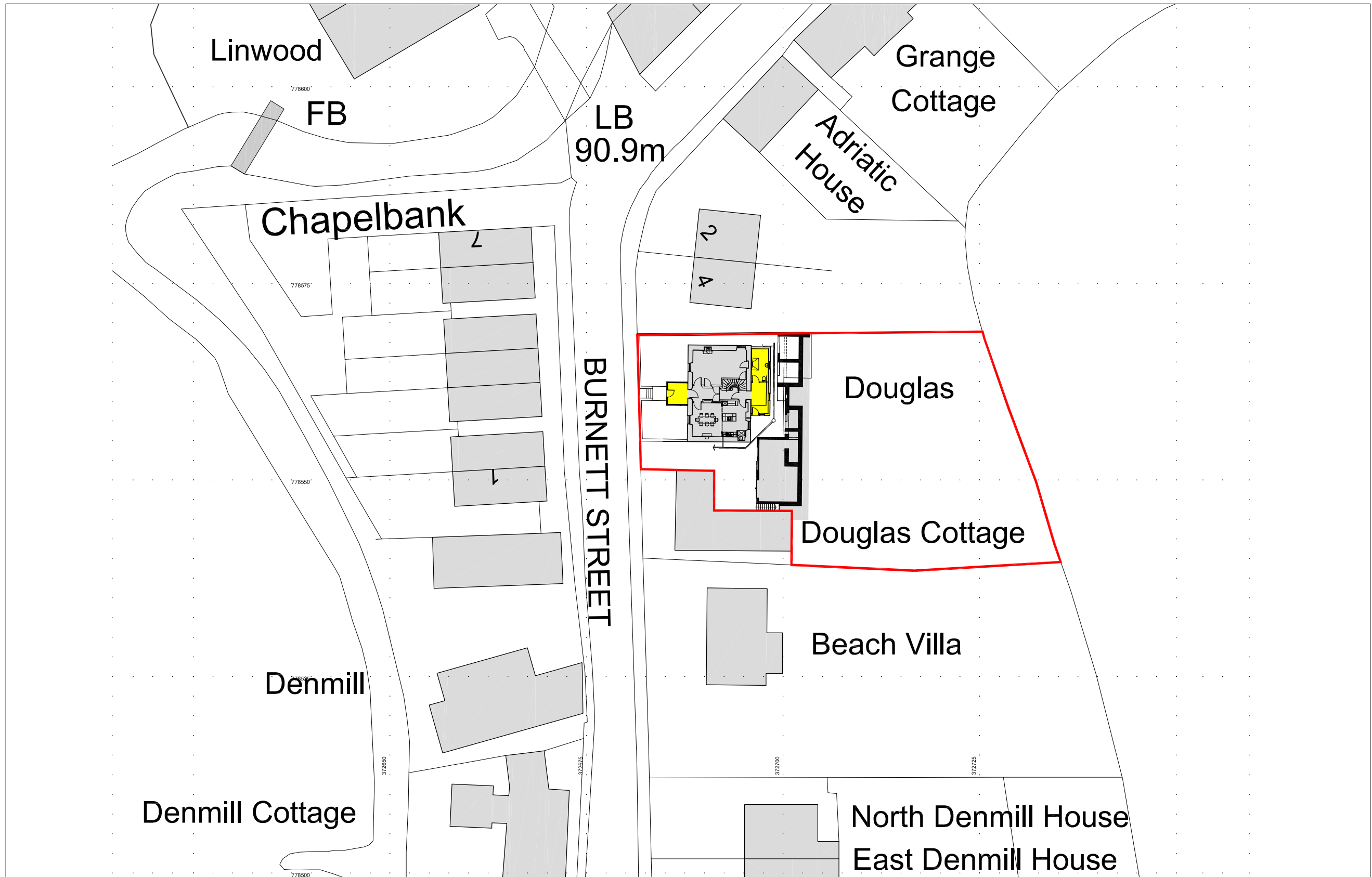
Existing Site Plan Scale 1:500
