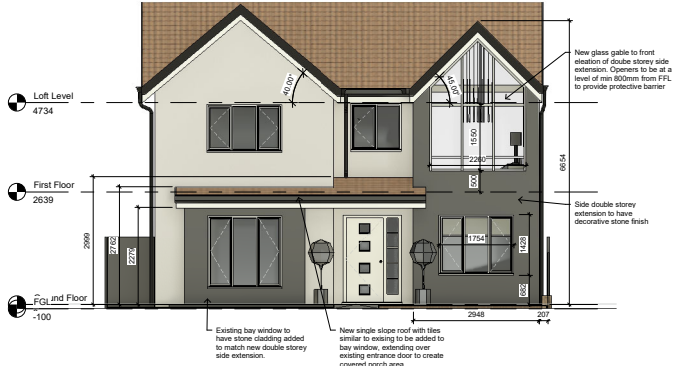
Proposed Front Elevation 1 : 50
