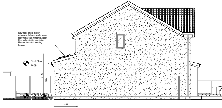
Proposed Side Elevation B 1 : 50
