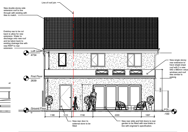
Proposed Rear Elevation 1 : 50
