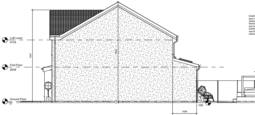
Proposed Side Elevation A 1 : 50
