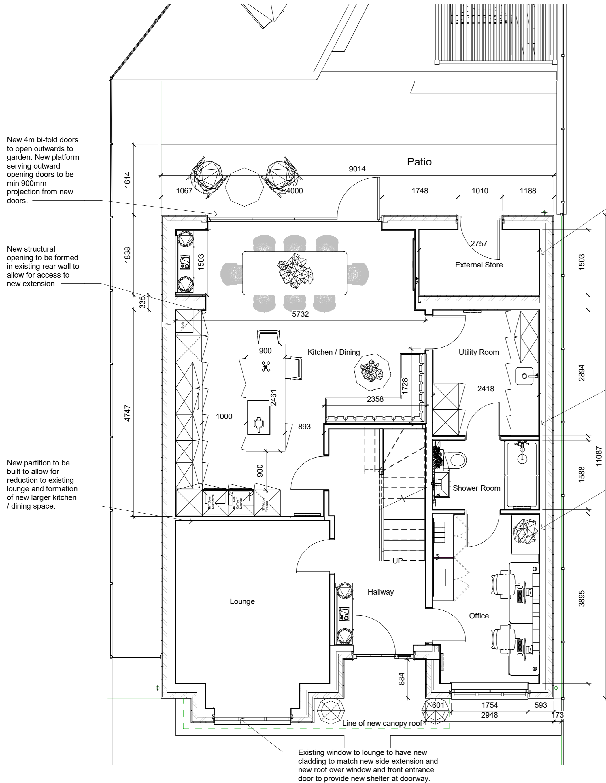
Proposed Ground Floor 1 : 50
