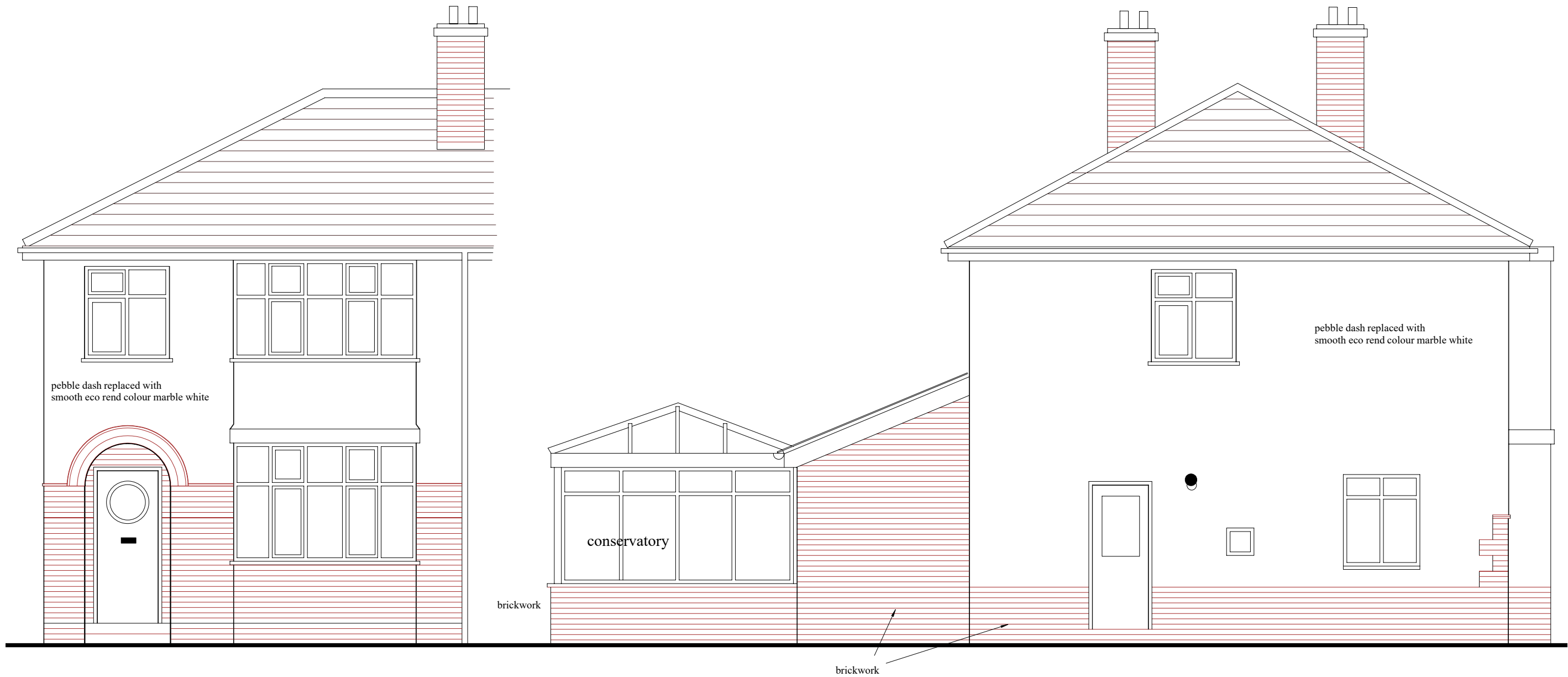
FRONT ELEVATION PROPOSED NORTH EAST
