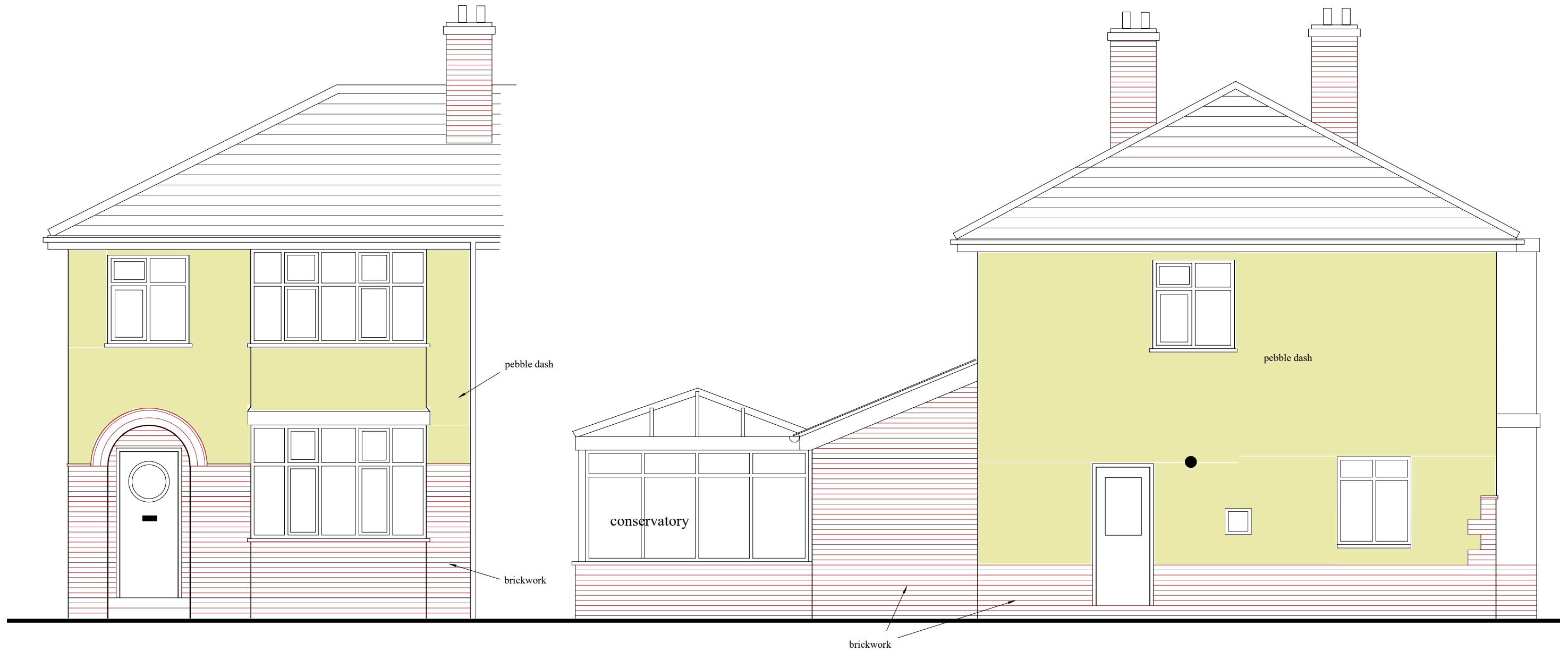
FRONT ELEVATION EXISTING NORTH EAST
