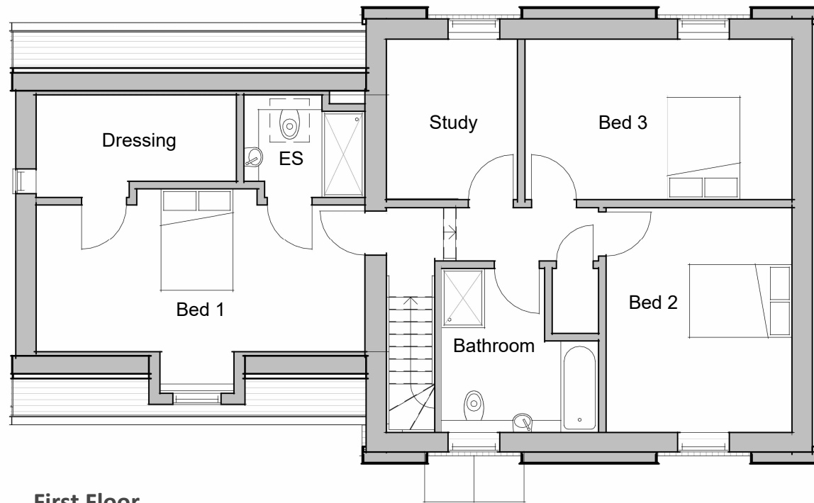
First Floor 1 : 100
