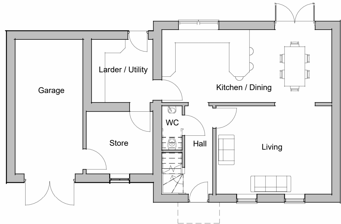
Ground Floor 1 : 100
