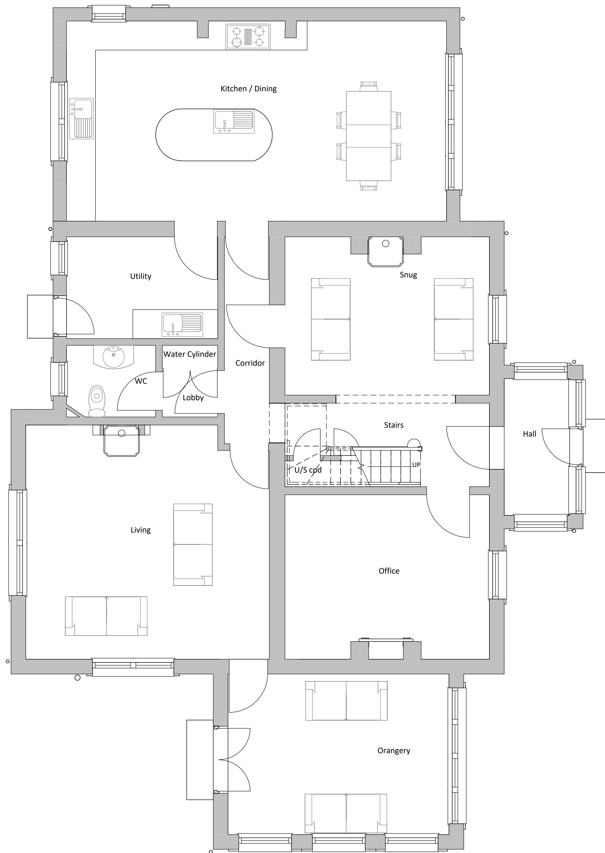
Existing Plan Level 00 1 : 50
