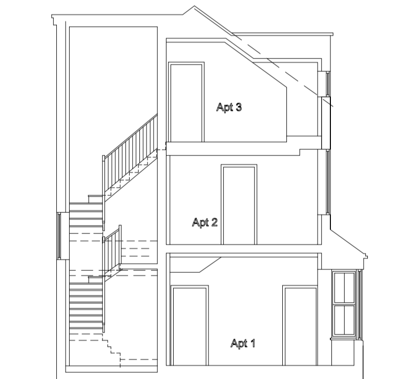
Section BB - No.54
