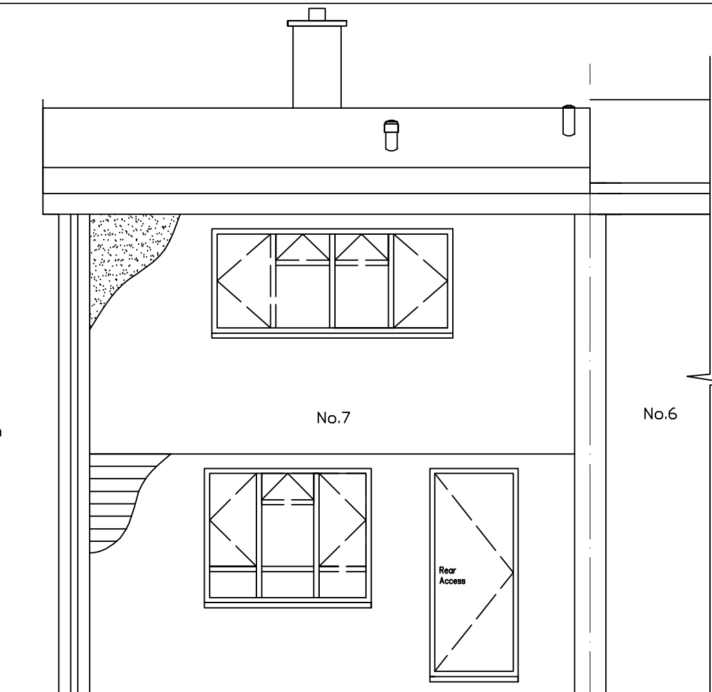
Rear Elevation
