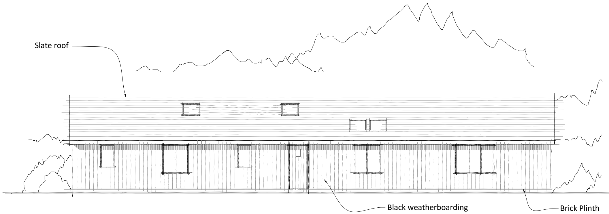
Rear Elevation
