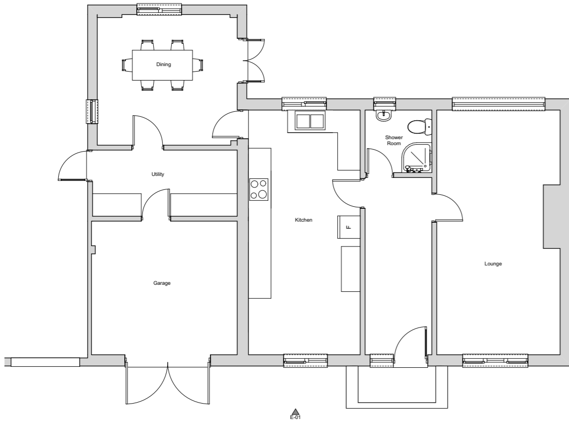
Existing Ground Floor Plan 1:100 - A3
