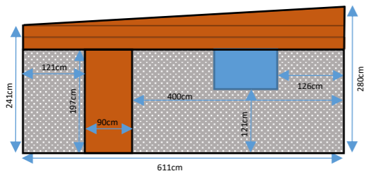
South Side View Current Scale 1:100
