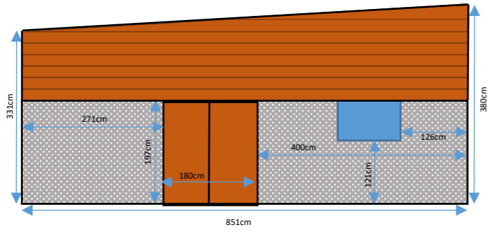
South Side View Proposed Scale 1:100
