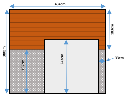
Front View Proposed Scale 1:100
