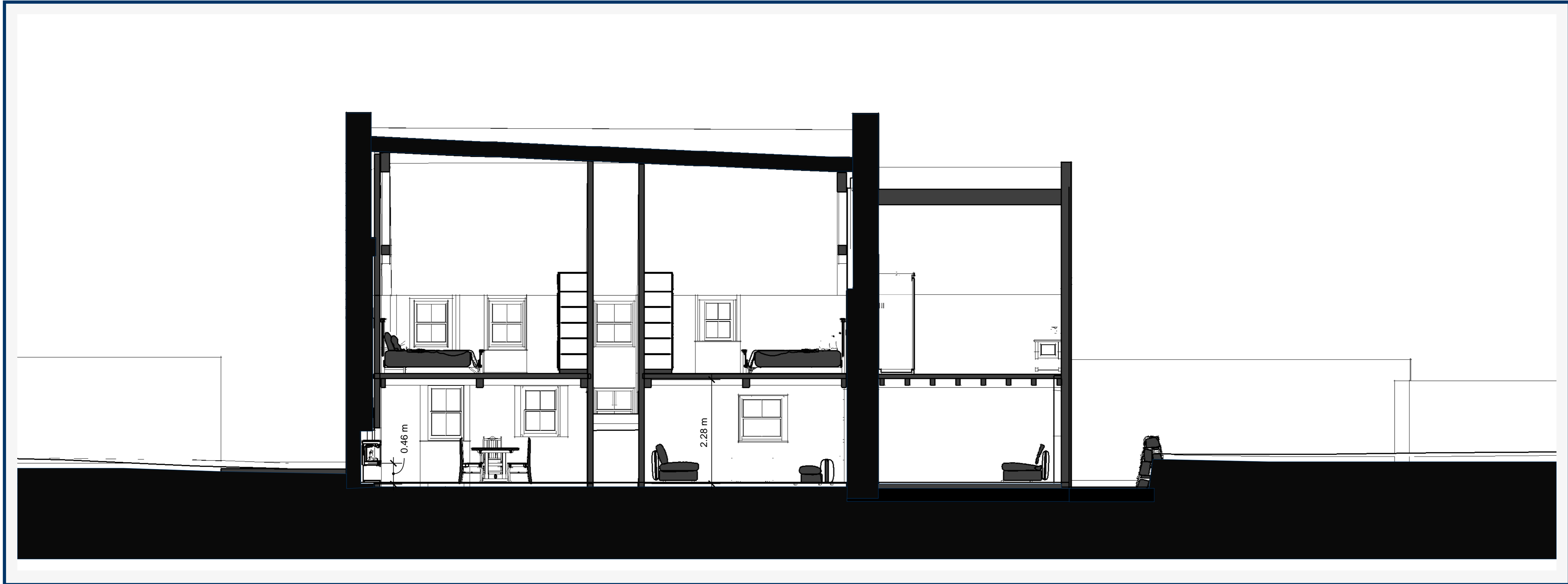
G Proposed Section 3 A3.8 1:50 @ A1
