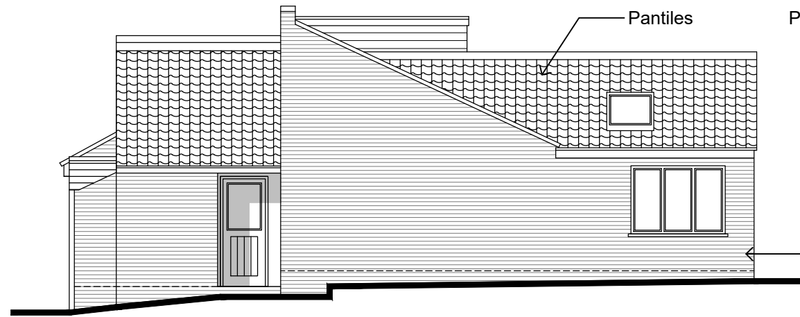
Existing North Elevation (1:100 scale)
