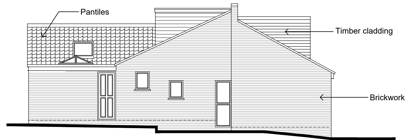
Existing South Elevation (1:100 scale)
