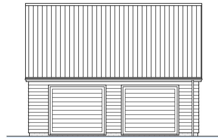
South Elevation 1:100
