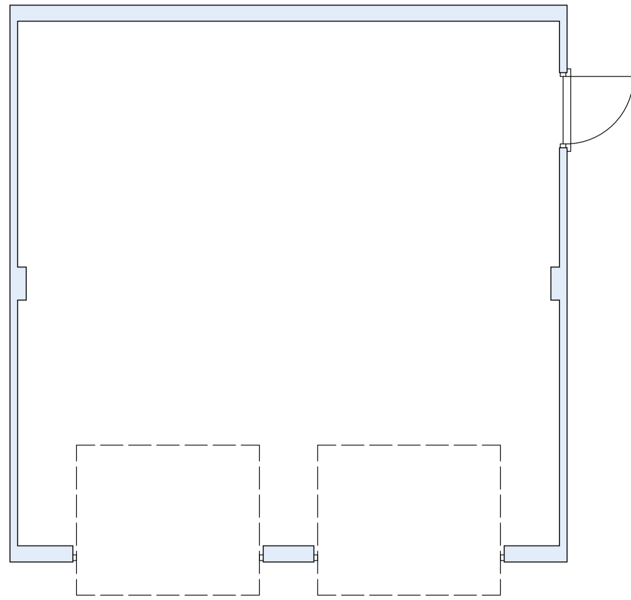
Garage Floor Plan 1:50
