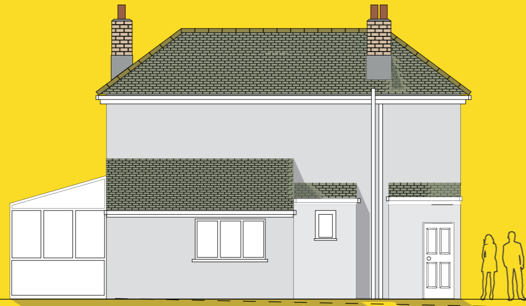
EXISTING FRONT ELEVATION (North facing)
