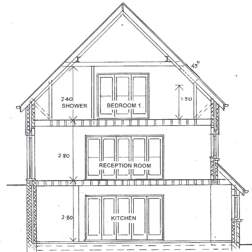
SECTION YY
