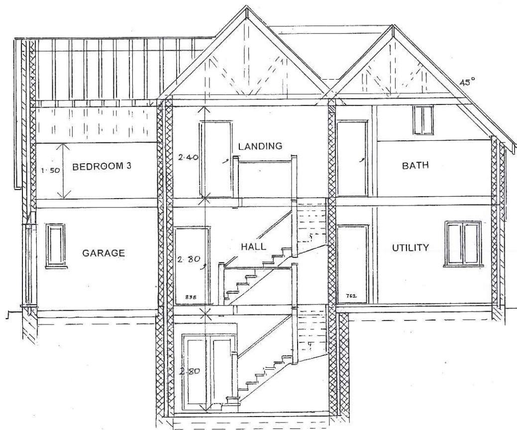
SECTION XX
