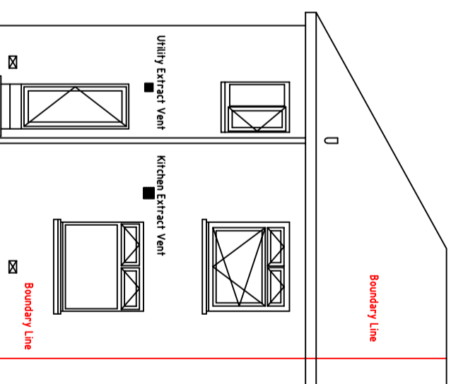
EXISTING REAR ELEVATION (SOUTH)
