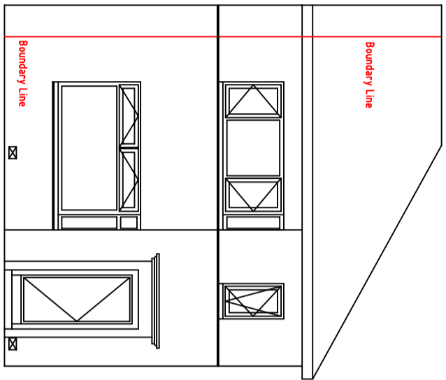
EXISTING FRONT ELEVATION (NORTH)
