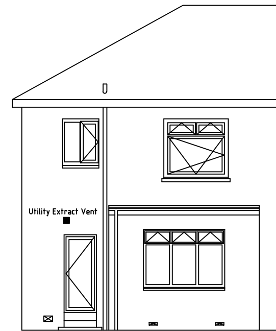
PROPOSED REAR ELEVATION (SOUTH)
