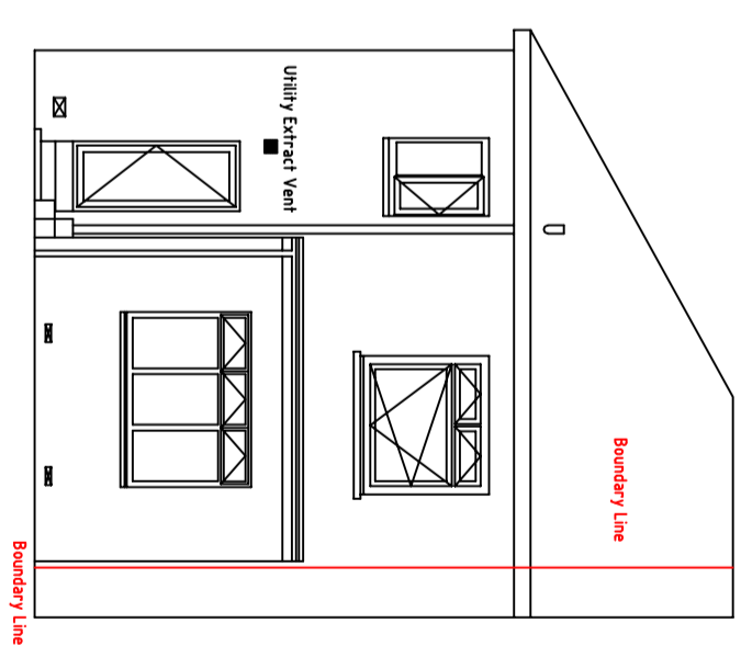
PROPOSED REAR ELEVATION (SOUTH)
