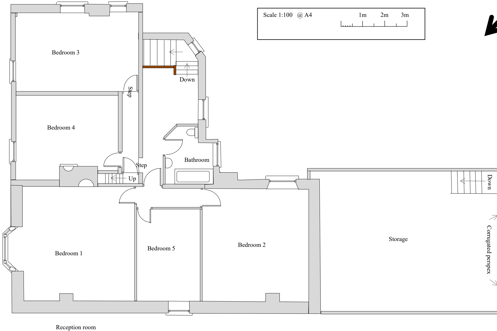
First floor plan (no heating)
