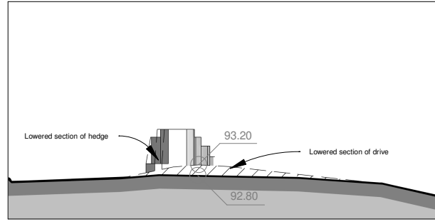
Section 1 - Proposed
