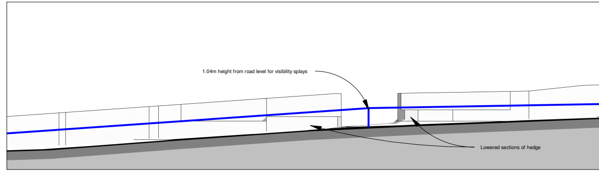
Section 2 - Proposed
