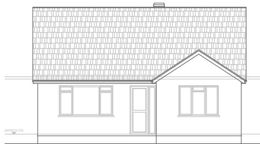
FRONT (NORTH WEST) ELEVATION
