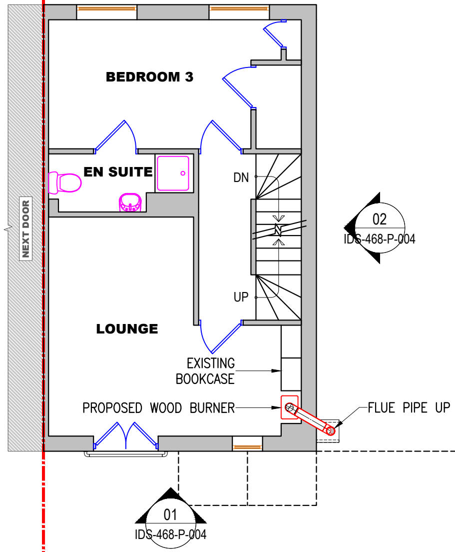
1 PROPOSED FIRST FLOOR LAYOUT Scale: 1:75
