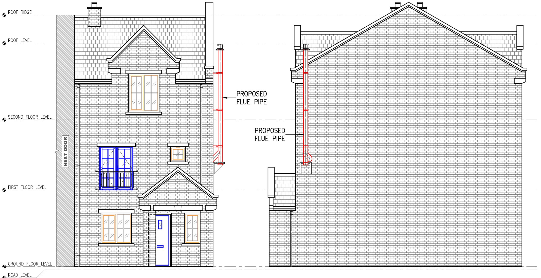
01 PROPOSED NORT-WEST ELEVATION Scale: 1:75
