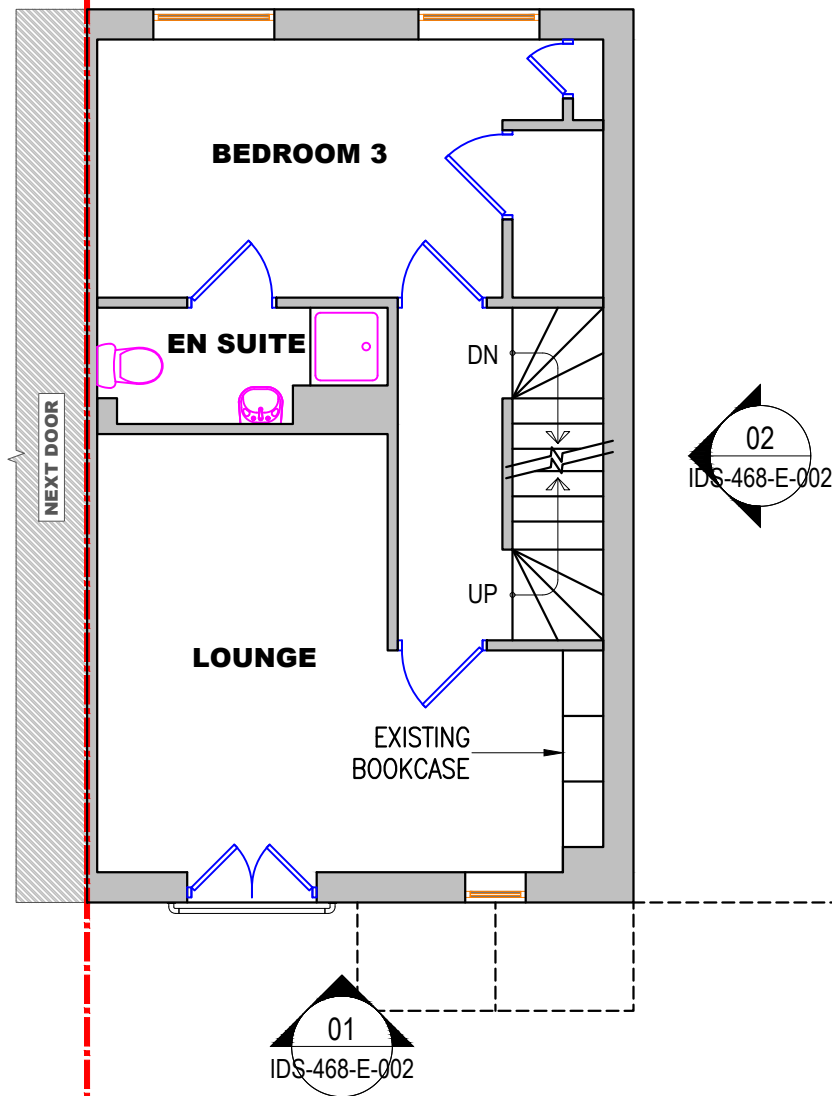
1 EXISTING FIRST FLOOR LAYOUT Scale: 1:75
