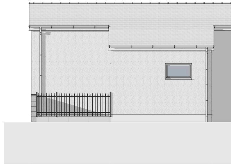
E 1 :: EXISTING FRONT ELEVATION scale: 1:100
