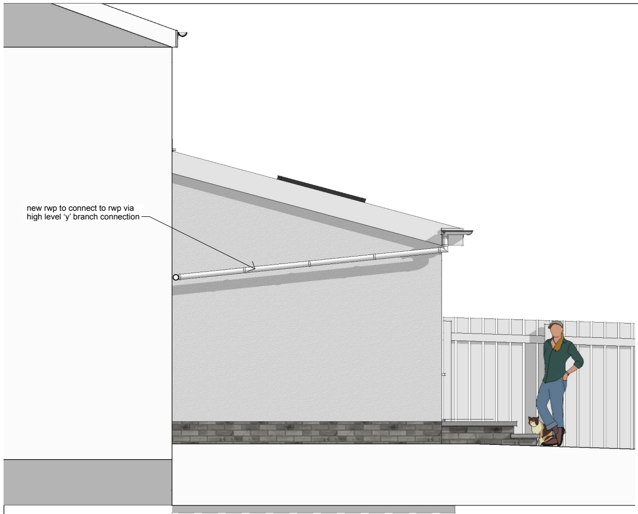
P :: PROPOSED SIDE ELEVATION 6 scale: 1:50
