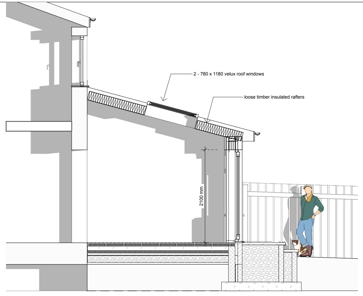
P :: PROPOSED SECTION 6 scale: 1:50
