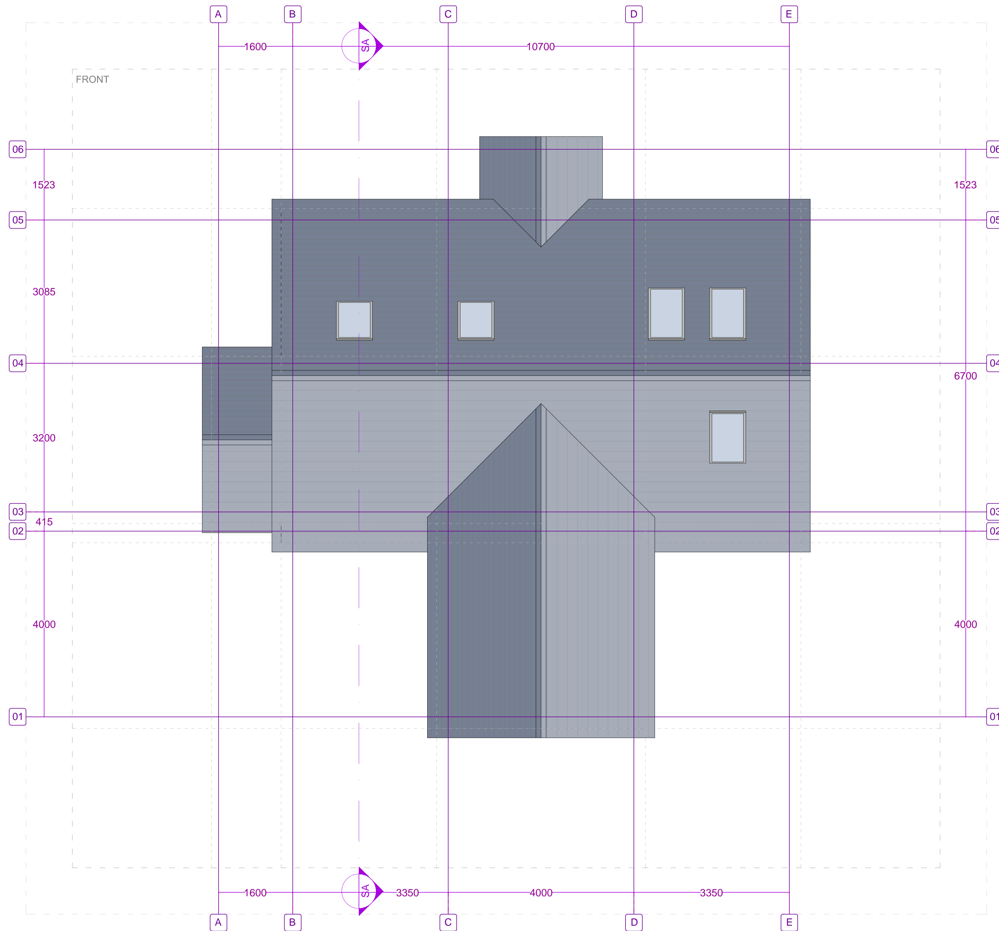
03 Proposed Roof Plan GA
