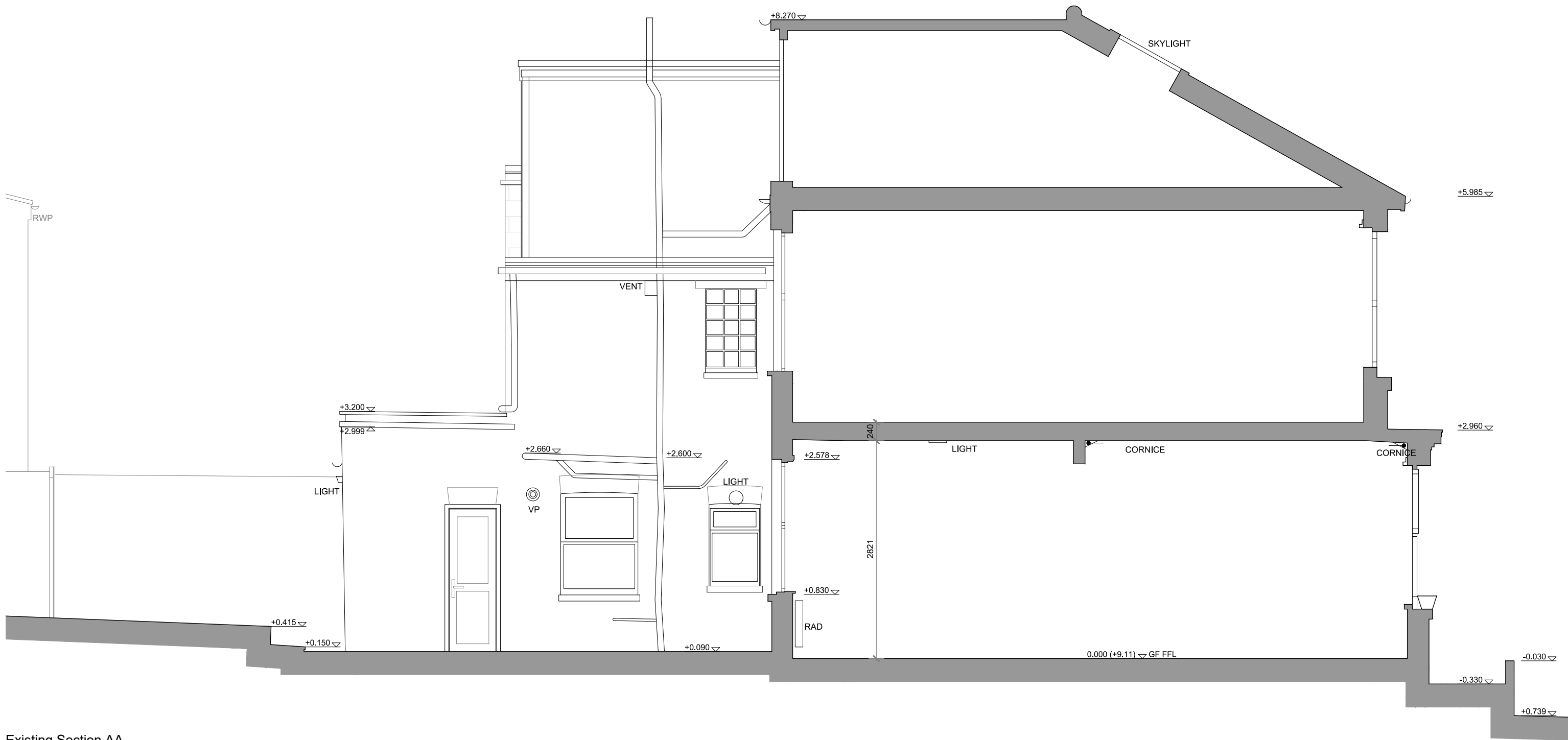
Existing Section AA 1:50
