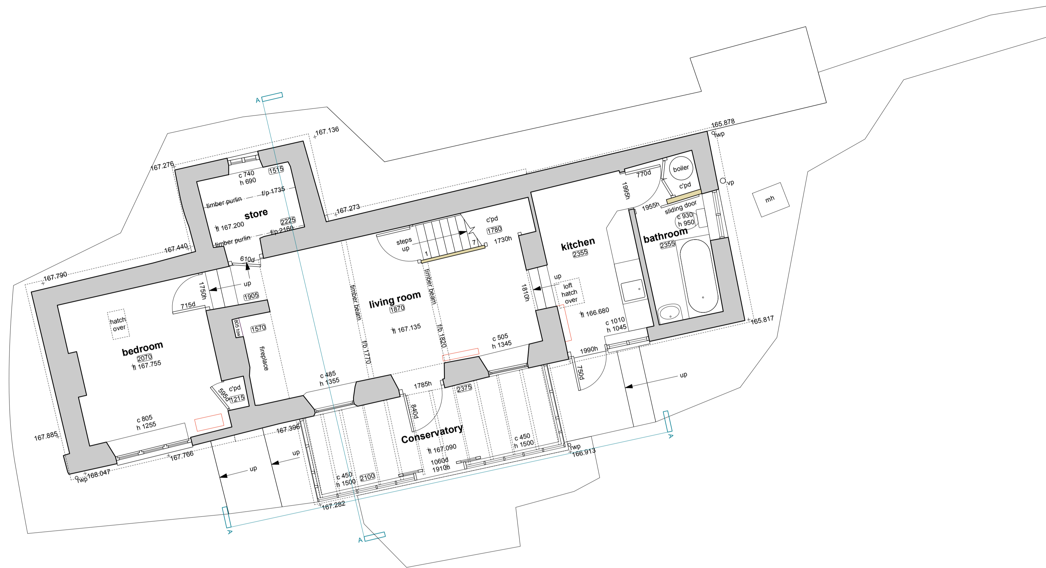
Existing Ground Floor Plan 1:50
