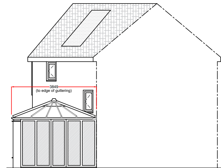
RIGHT-HAND SIDE ELEVATION
