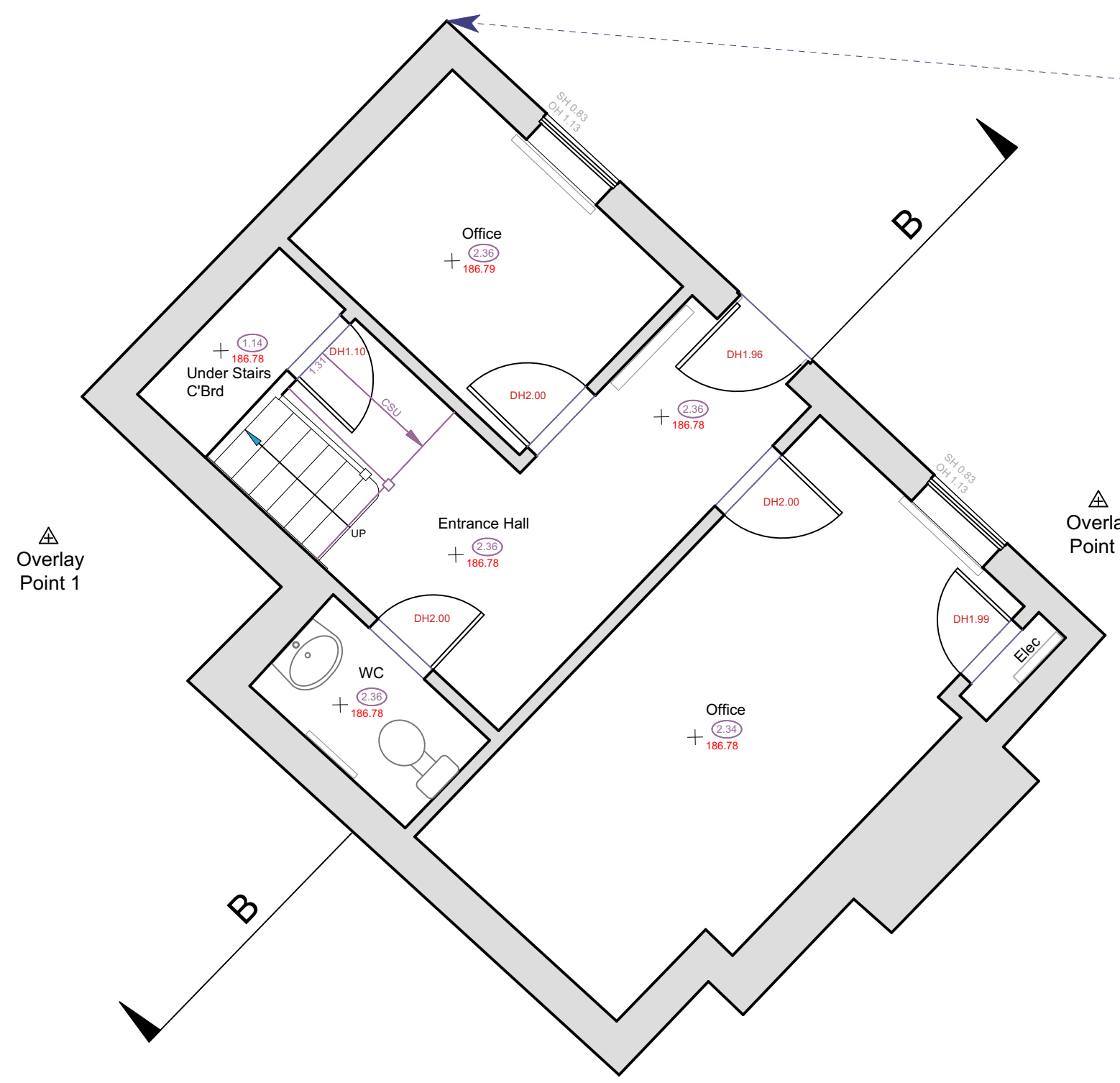
Lower Ground Floor Plan Scale : 1.50
