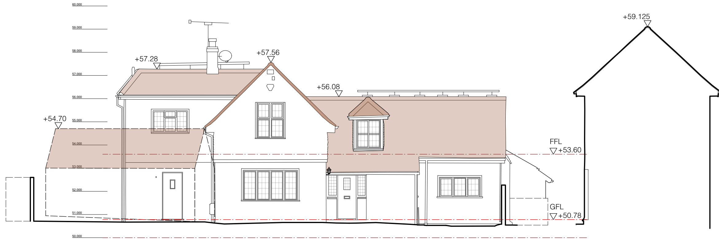
FRONT ELEVATION
